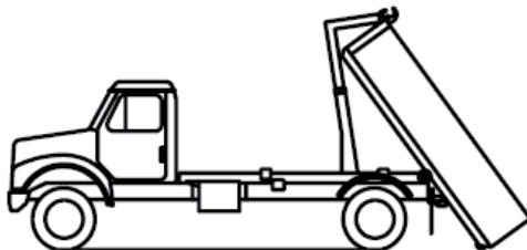
MAX. DUMPING ANGLE 54 DEG
